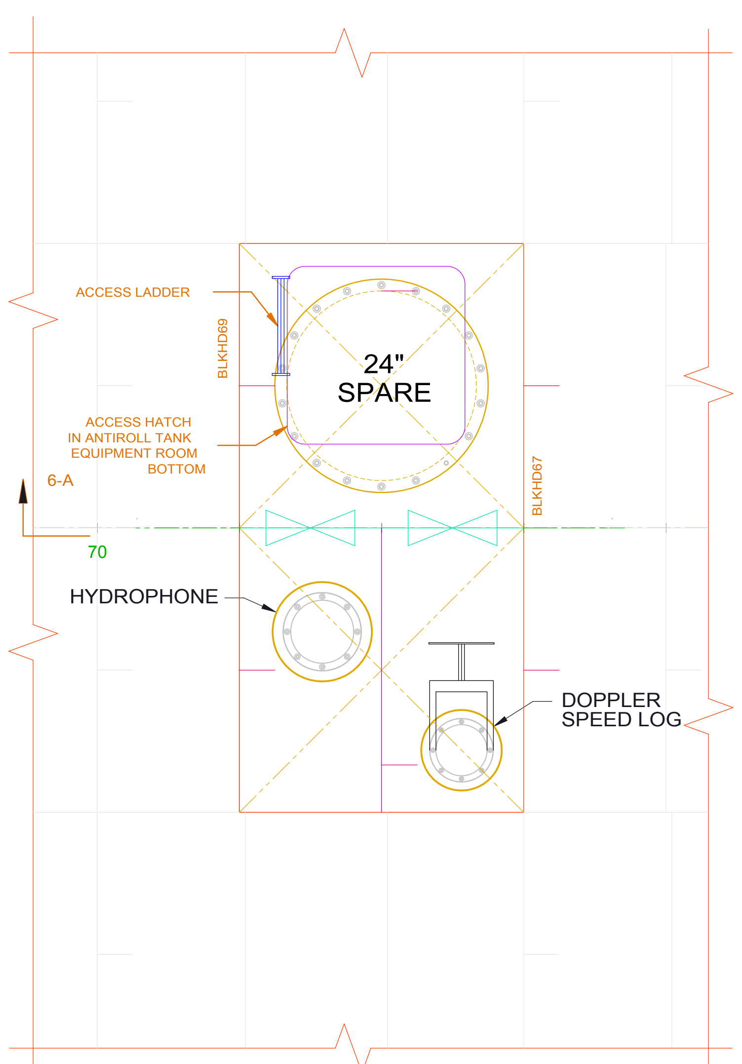
PLAN 15-C AFT TRANSDUCER WELL
