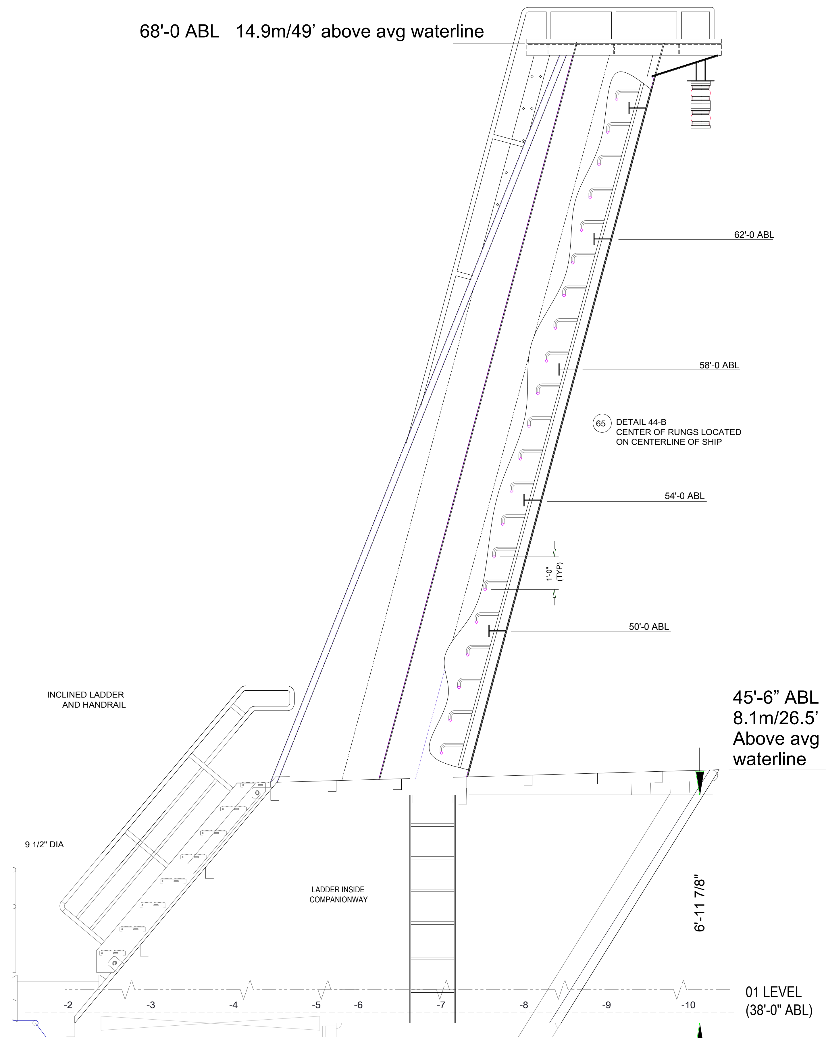
ELEVATION 43-A STEEL FORWARD MAIN MAST LKG PORT SCALE 3/4" = 1'-0"
